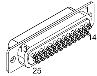
25 PIN MALE D-STYLE, ECK00101 BACKSHELL, ECK0656
