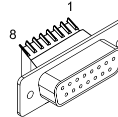
15 LINE FEMALE "D", ECK00783 BACKSHELL, ECK01022
