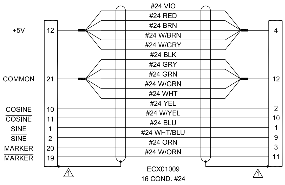
26HD MALE, ECK01259 BACKSHELL, ECK01022
