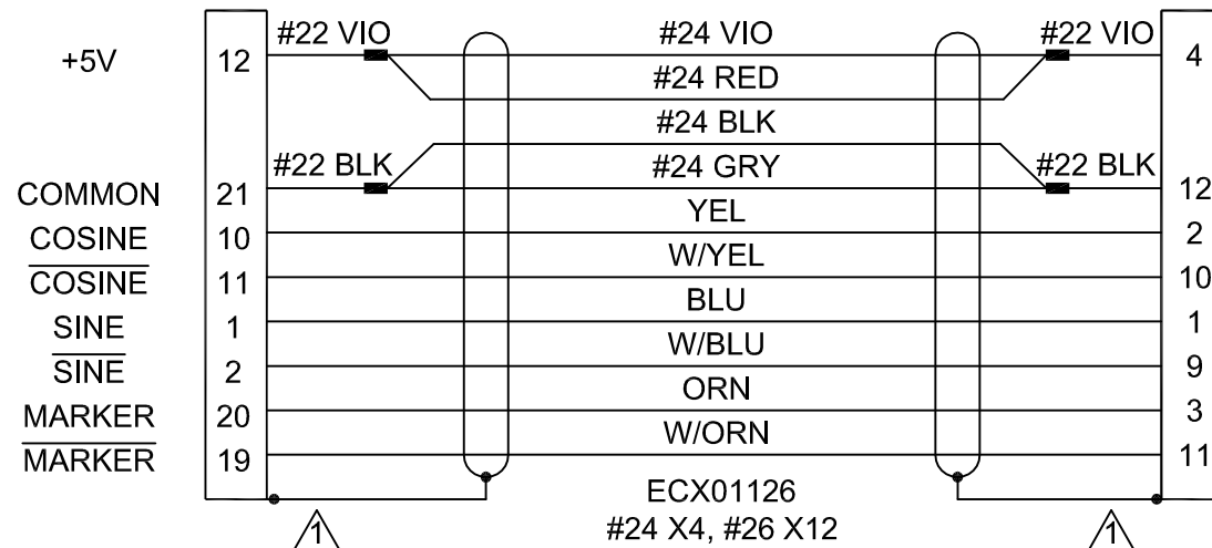
15 LINE FEMALE "D", ECK00783 BACKSHELL, ECK01022
