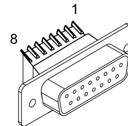
15 LINE FEMALE "D", ECK00783 BACKSHELL, ECK01022
