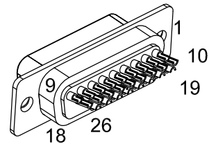
26HD MALE, ECK01259 BACKSHELL, ECK01022
