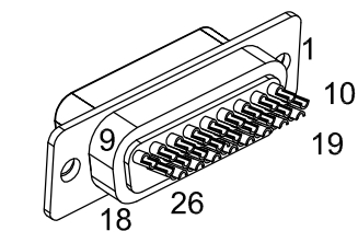
26HD MALE, ECK01259 BACKSHELL, ECK01022
