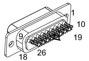
26 HD MALE, ECK01259 BACKSHELL, ECK01022
