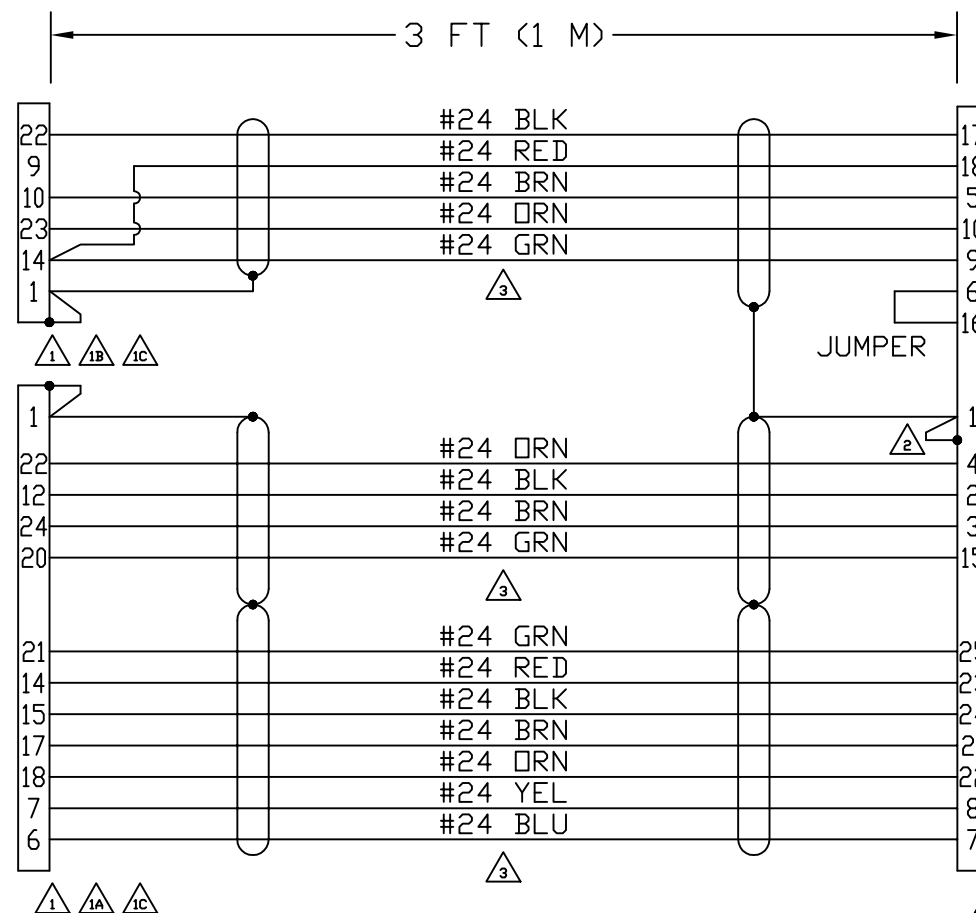
ASSEMBLY OUTLINE
