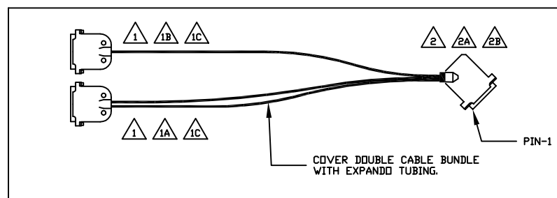
ASSEMBLY OUTLINE
