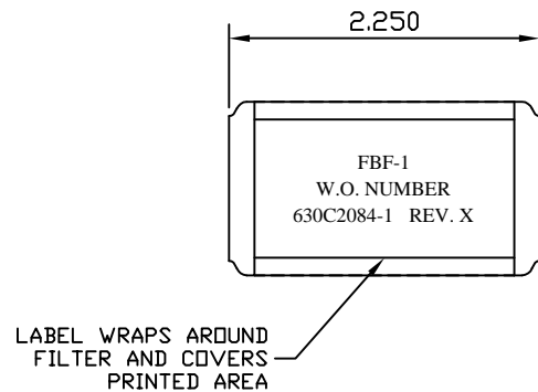
SIDE VIEW OF FERRITE BEAD ASSEMBLY COMPLETED
