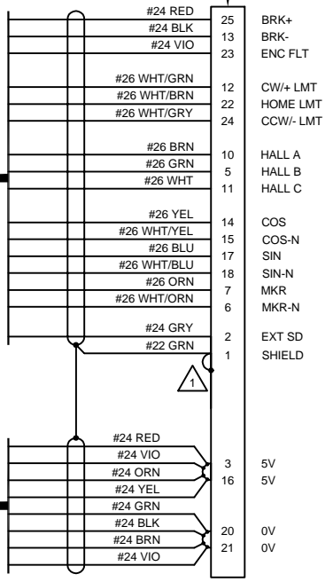
DETAIL-B DB25S (ECK00300) VIEW: WIRING SIDE
