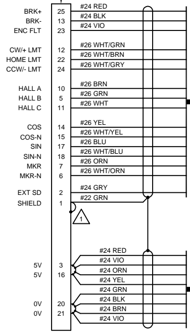
DETAIL-A DB25P (ECK00101) VIEW: WIRING SIDE
