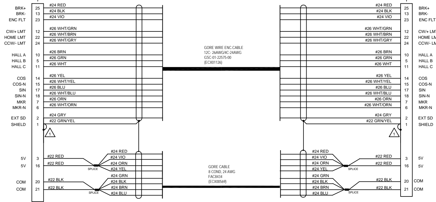
DETAIL-A DB25P (ECK00101) VIEW: WIRING SIDE
