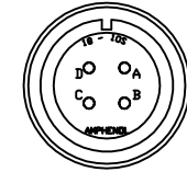
DETAIL "A" VIEWED FROM WIRE SIDE OF CONNECTOR AMPHENOL SOCKET INSERT MS18-10S (MCM495)
