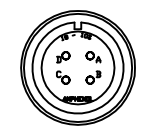
DETAIL "A" VIEWED FROM WIRE SIDE OF CONNECTOR AMPHENOL SOCKET INSERT MS18-10S (MCM495)
