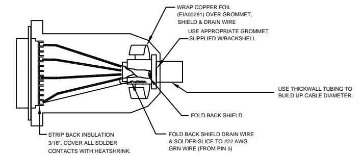
2 SOCKET, 14 PIN, 206043-1 AMP SQ FLANGE-ROHS (ECK00130) AND STRAIN RELIEF 206070-8 AMP (ECK00134) CONNECTOR DETAILS
