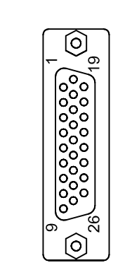
VIEW FROM SOLDER SIDE
