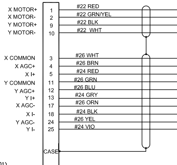
WIRING SIDE VIEW
