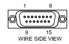
DB15S ECK00783 BACK SHELL ECK01022
