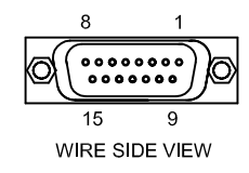
15 PIN MALE D, ECK00790 BACKSHELL ECK01022
