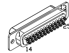
25 PIN D-FEMALE, ECK00300 BACKSHELL, ECK01057
