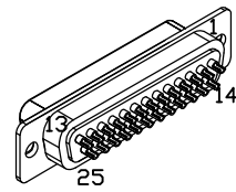
25-PIN D-MALE, ECK00101 BACKSHELL, ECK01057
