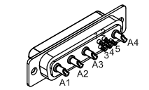
HPD FEMALE "D", ECK00657 SOCKET CONTACT, ECK00659 BACK SHELL, ECK00656
