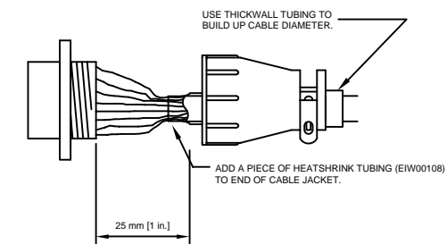
2 SOCKET, 14 PIN, 206043-1 AMP SQ FLANGE-ROHS (ECK00130) AND STRAIN RELIEF 206070-8 AMP (ECK00134) CONNECTOR DETAILS
