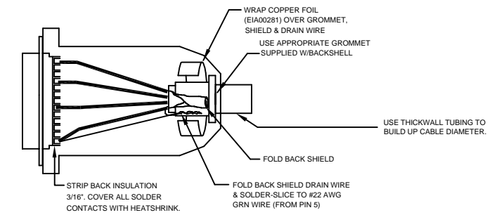
1 CONNECTOR HI-PWR-'D' 5 PIN MALE ITT CANNON DBM5W5PK87 (ECK01236) CONNECTOR DETAILS
