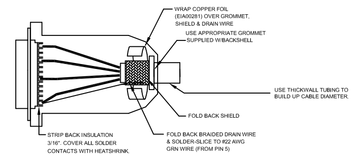
2 SOCKET, 14 PIN, 206043-1 AMP SQ FLANGE-ROHS (ECK00130) AND STRAIN RELIEF 206070-8 AMP (ECK00134) CONNECTOR DETAILS
