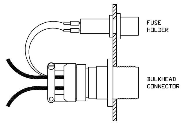
TYPICAL MOUNTING OF CONNECTOR & FUSE HOLDER
